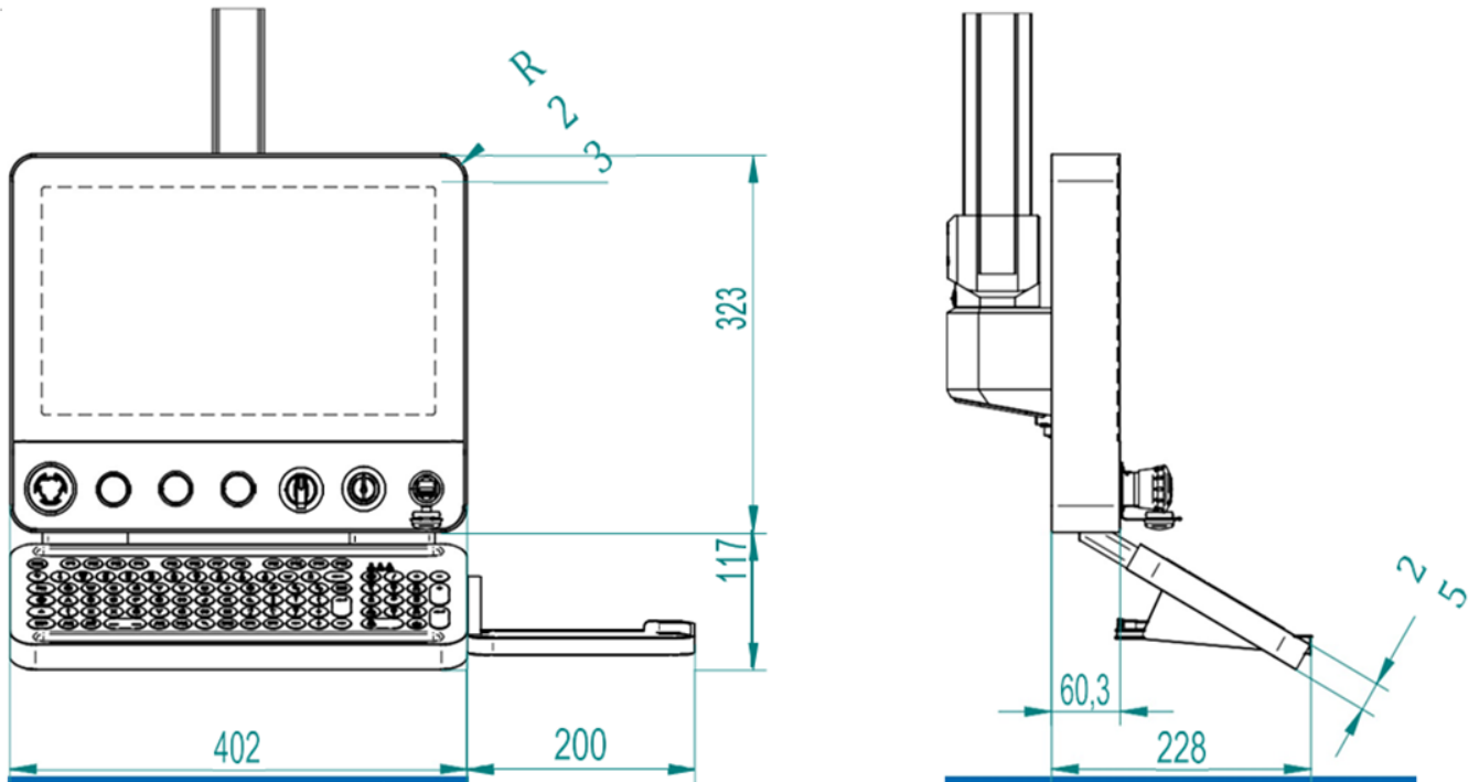
Example push-button panel for references
